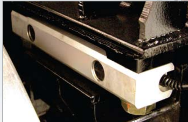
Under-Body Mount Load Cell
